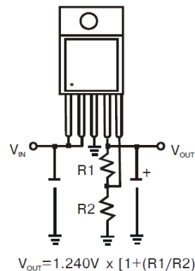
Figure2. Adjustable output voltage configuration. For best results, the total series resistance should be small enough to pass the minimum regulator load current
